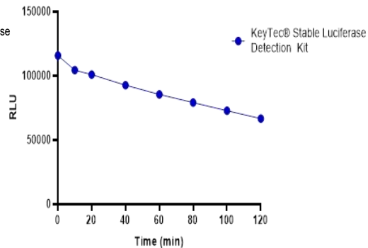
NF-KB Hek293 cells
