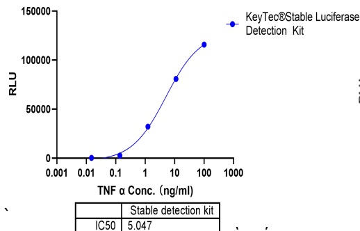
TNF \alpha Dose Response Curve
