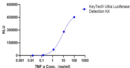
TNF \alpha Dose Response Curve
